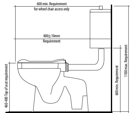
SEAT HEIGHT
